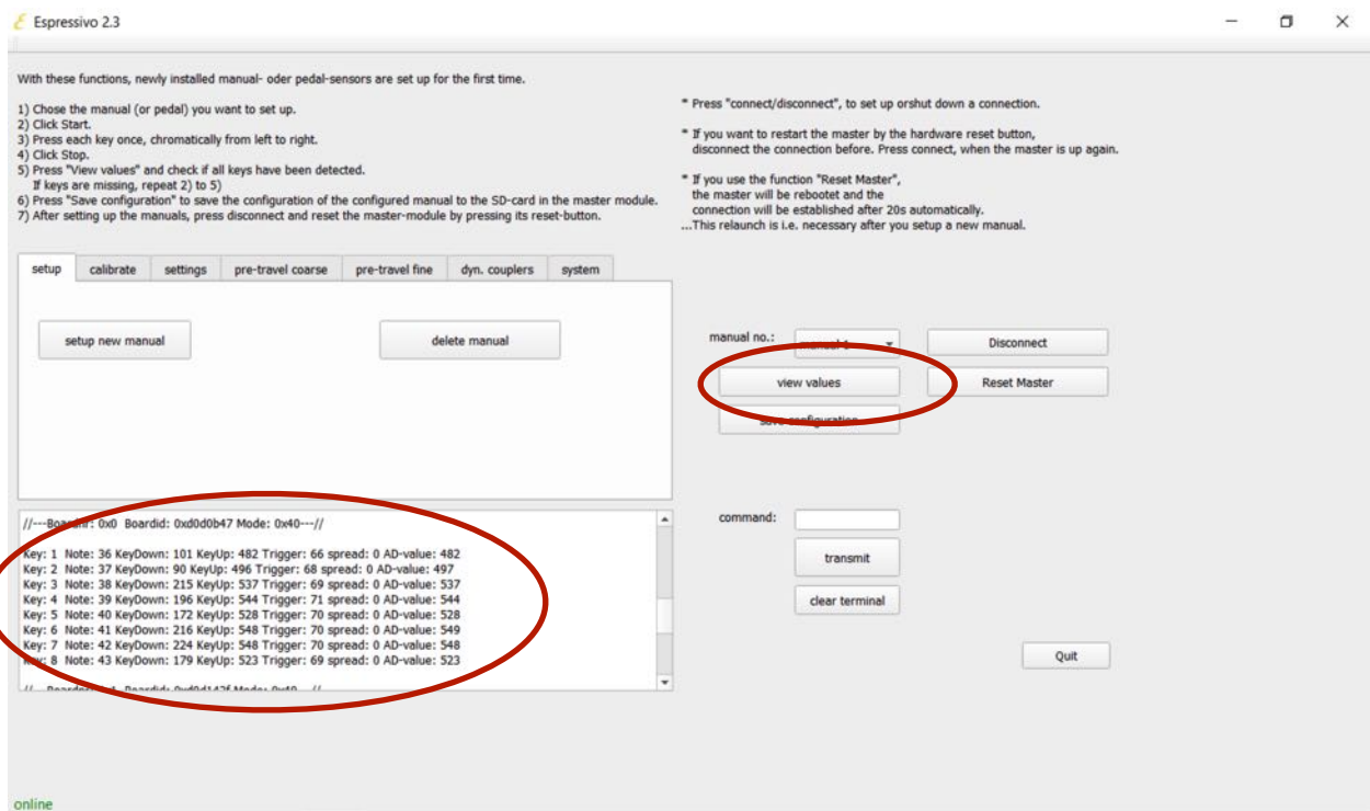
Display of sensor values in the terminal window
