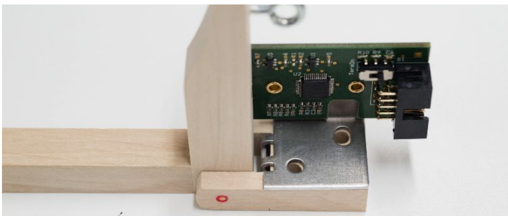
Single Espressivo sensor with mounting bracket, magnet and square
